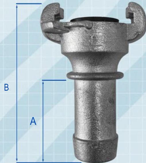
A-Claw Hosetail
